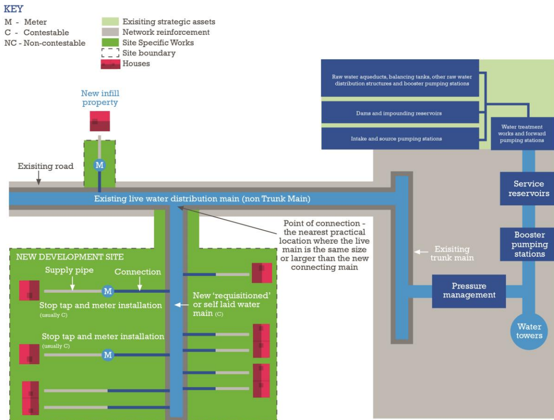
Figure 1 - Water Network
