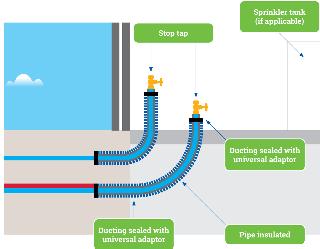
Stop tap (to be installed on both domestic and fire supply)
